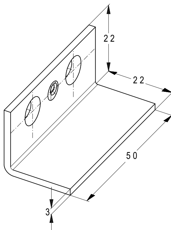
Winkel 22x22x50x3
